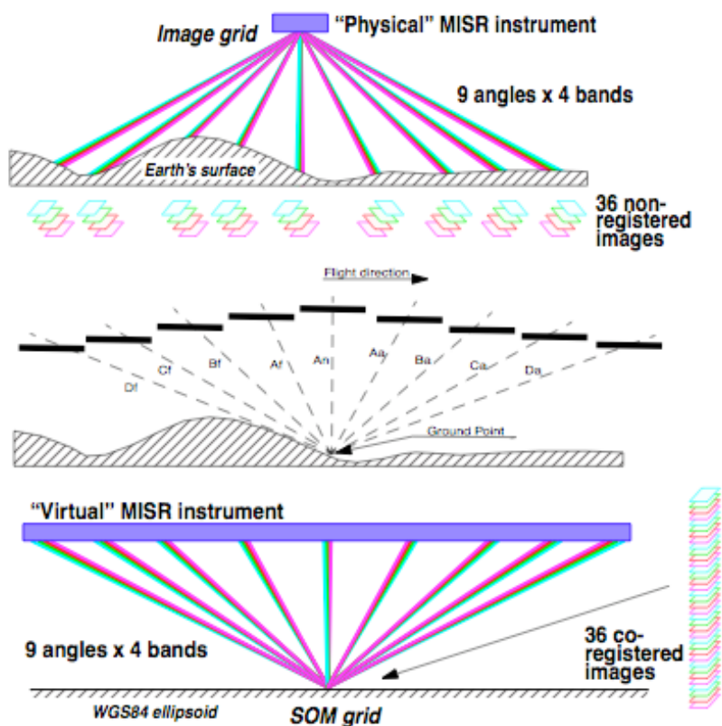
Figure A-2 Diagrams depicting the Multi-Angle concept
