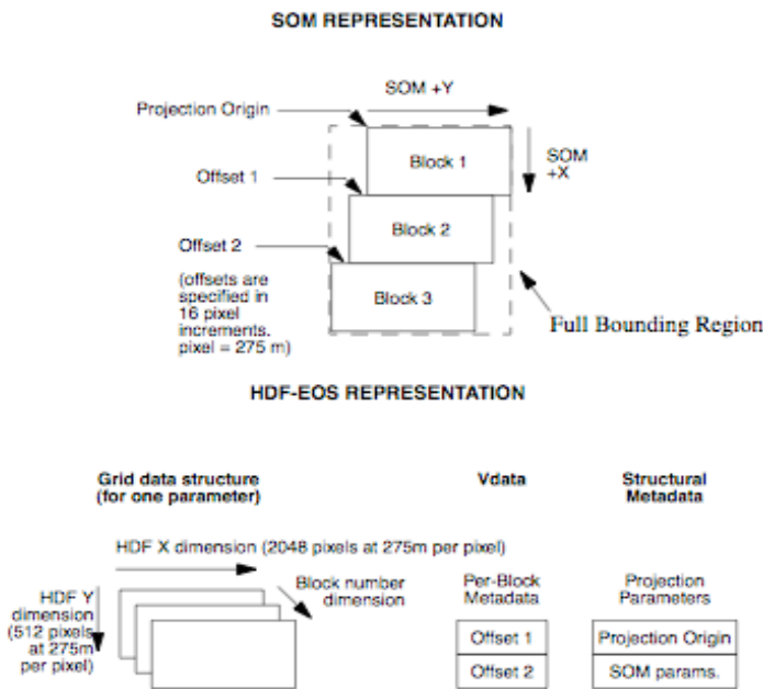
Figure 3-1 MISR SOM Representation in HDF-EOS
