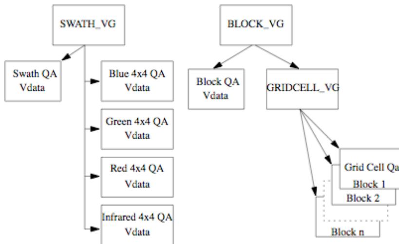
Figure 3-3 MISR QA special Grid Cell Vdata structures
