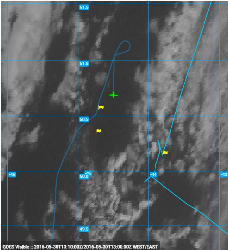
1320Z_HighAlt_N-S_Survey
