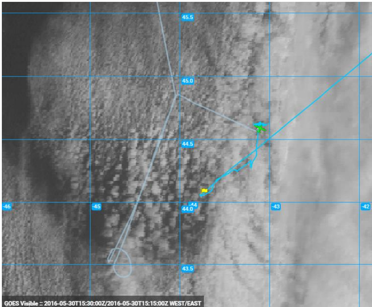
1545Z_LowLevelNearTheShip
