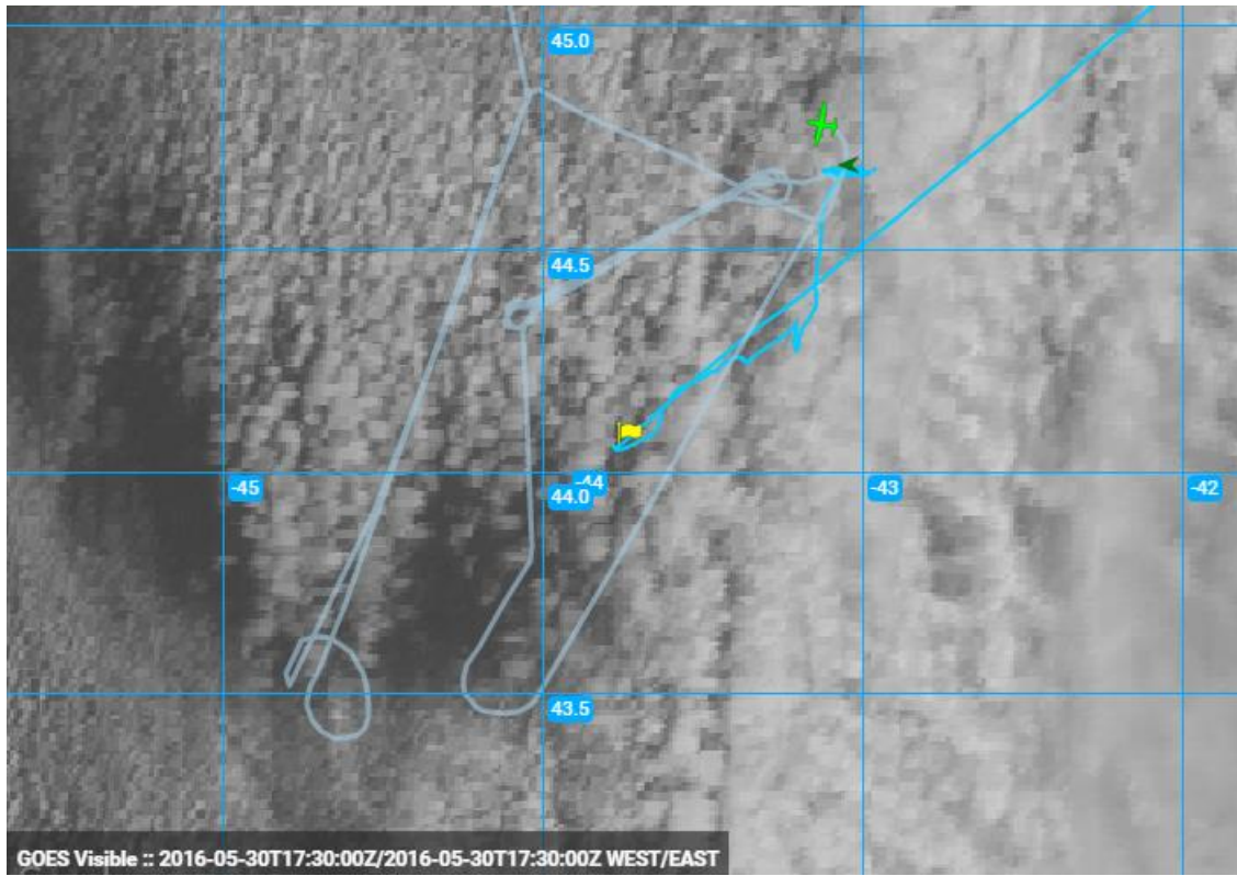
1740Z_SpiralDown
