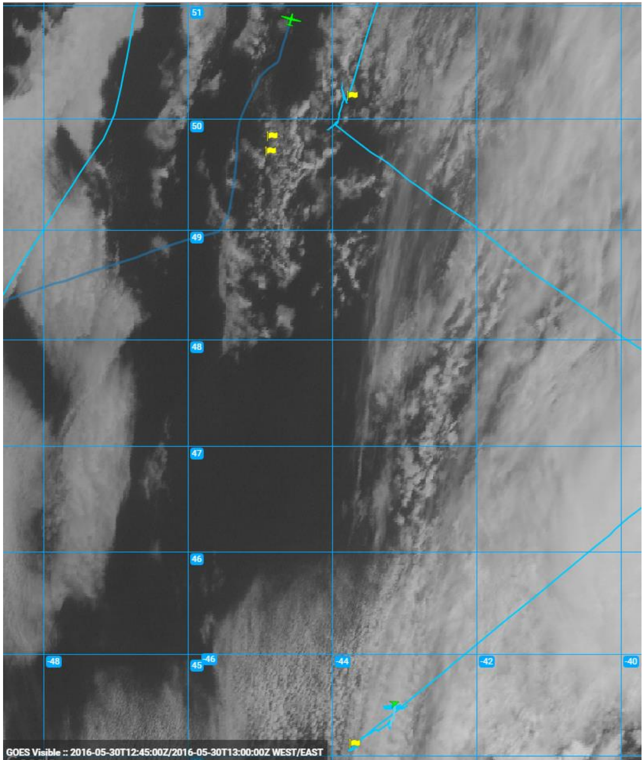
1310Z_LiningUpForHighAltSurvey
