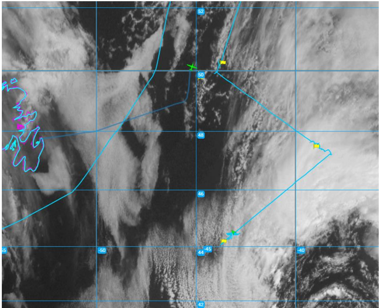
1300Z_LiningUpForHighAltSurvey
