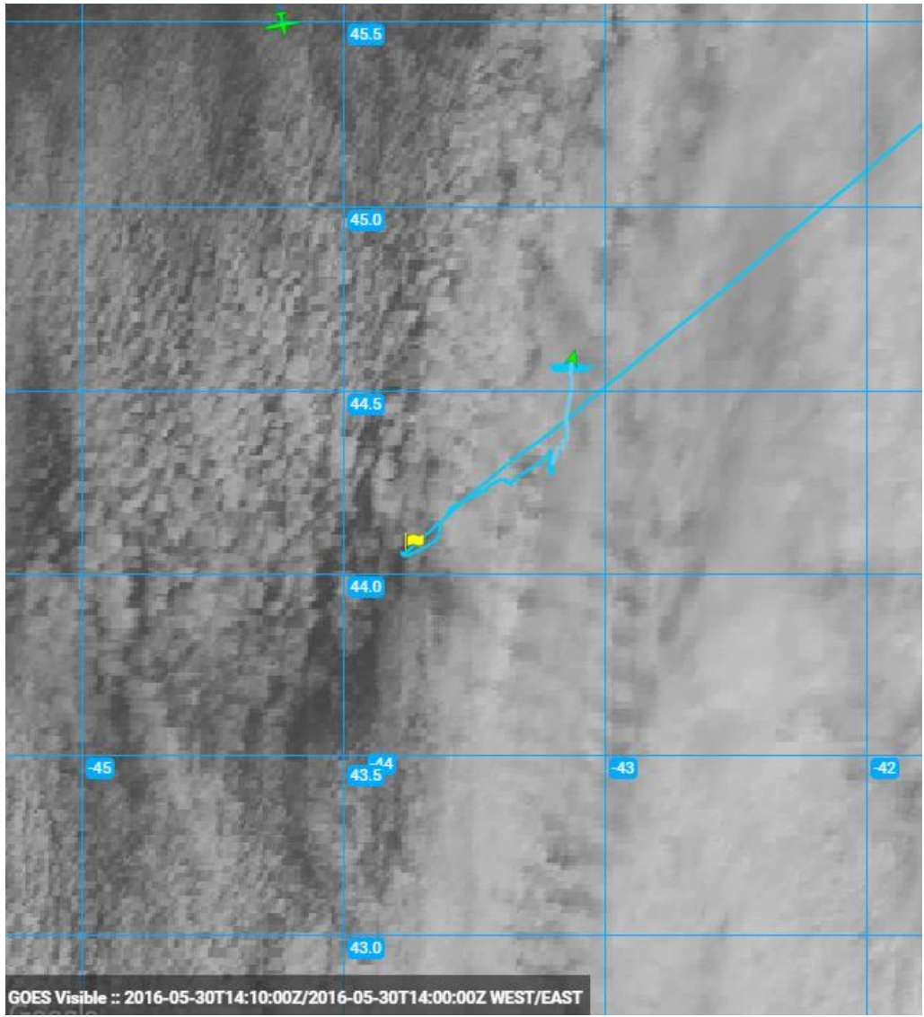
1425Z_ApproachingZpattern
