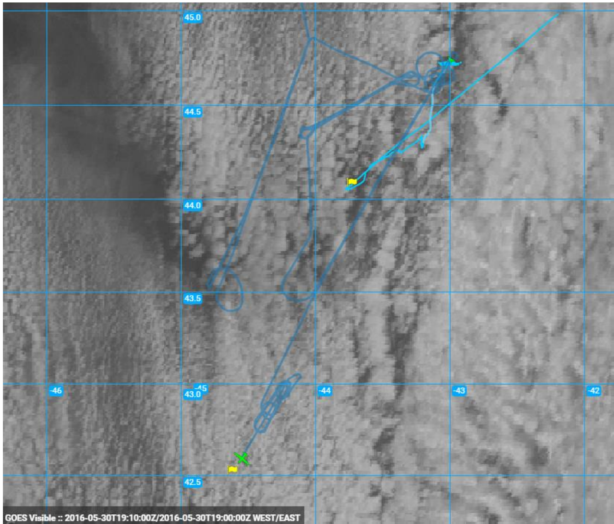
1920Z_SettingUpForCALIPSOTrack
