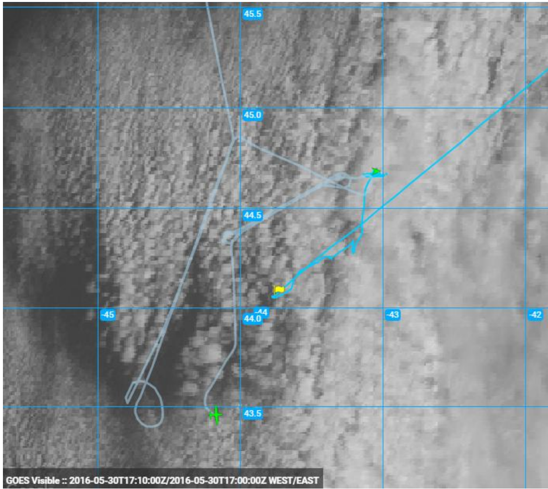
1720Z_SettingUpForHighAltZpattern
