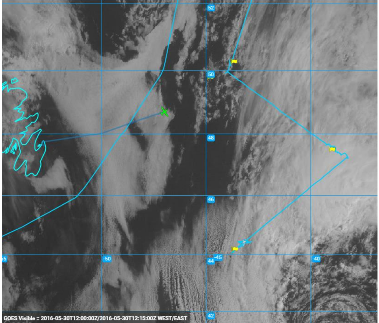
1230Z_HeadingOutToTheBox
