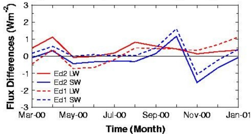
Monthly Global Mean, FM2 Minus FM1, All Sky Condition
