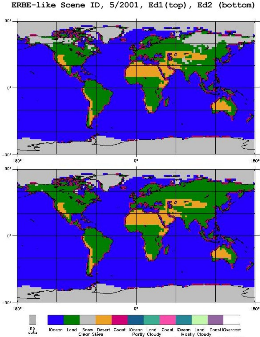
Figure 2. Comparison of monthly mean ERBE-like scene ID between Edition1 (top) and Edition2 (bottom) data product.
