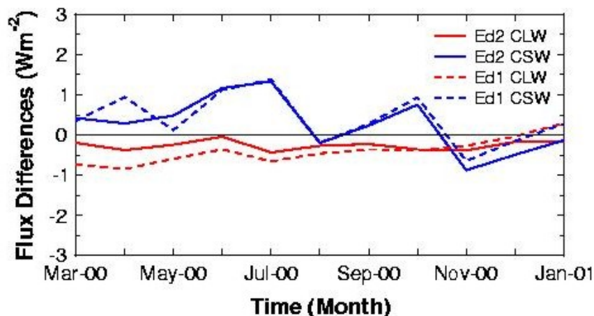
Figure 1. Comparison of global monthly mean FM1 and FM2 fluxes (FM2 minus FM1) between Edition1 and Edition2 data product.
