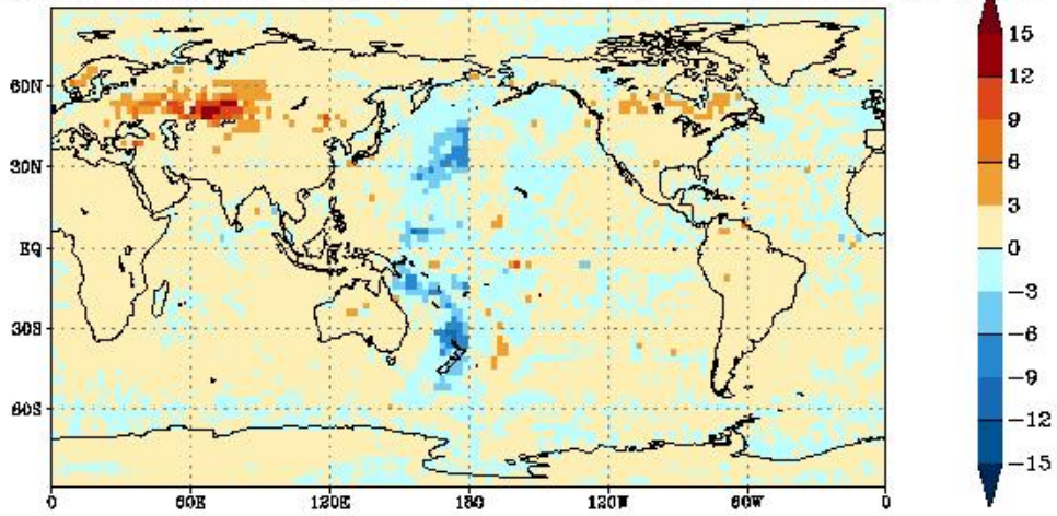
Figure 3. Differences (ed2 minus ed1) in monthly mean regional all-sky shortwave flux between Edition2 and Edition1 data product.
