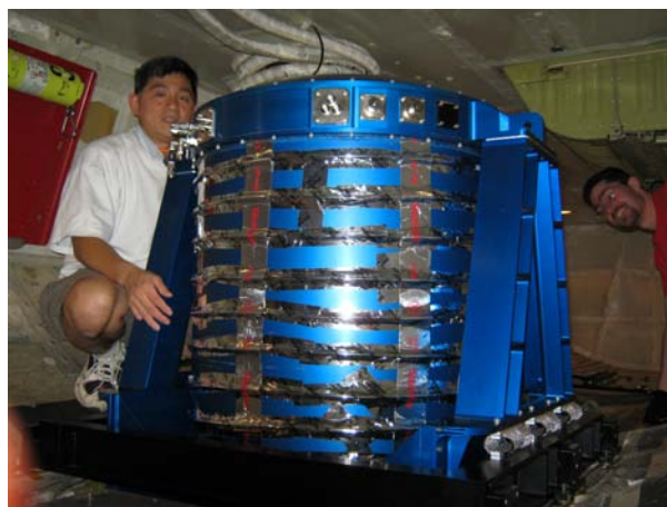
Fig. 2: The DAWN Lidar Optics Canister Containing Laser, Receiver, Telescope, and Scanner
