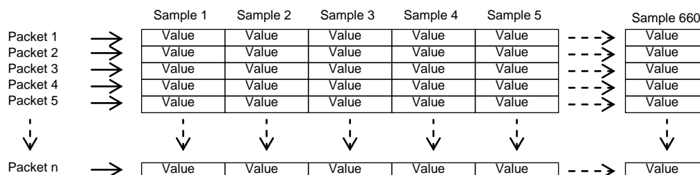
Figure 1. BDS SDS Schematic
